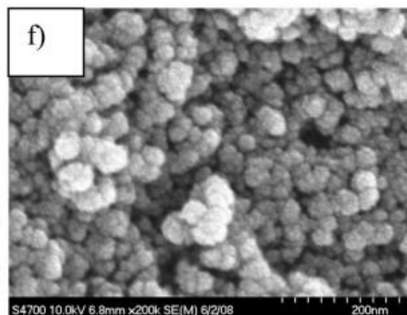
Figure 3.2d,f Underderivatized Silica Aerogel
